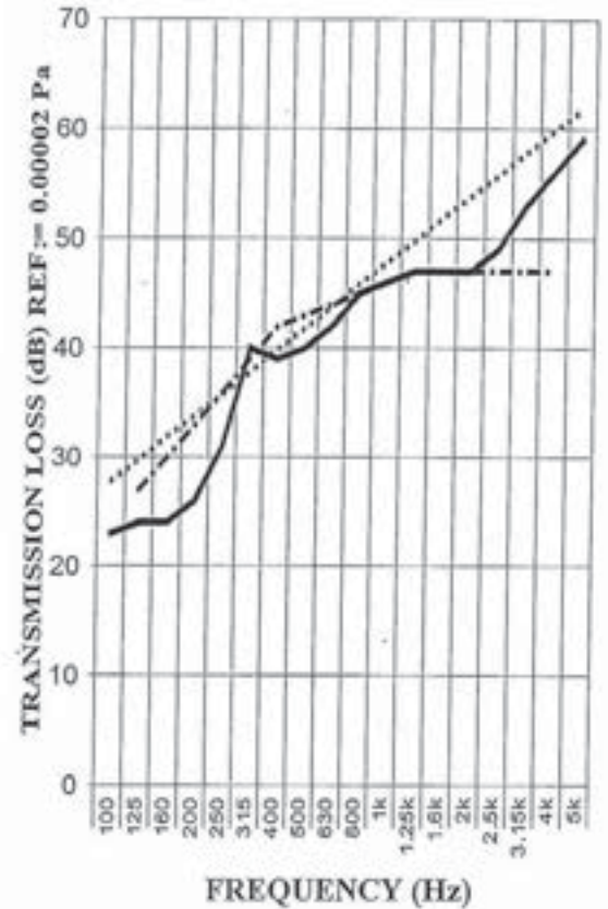
STC data for steel clad sound stop panels
