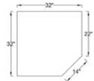
Corner Cabinet Plan View
